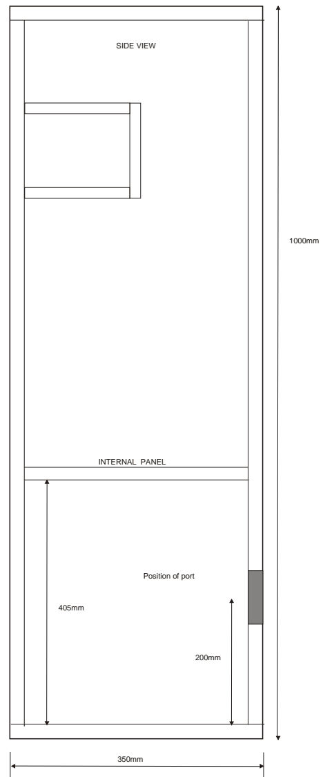
SIDE VIEW
